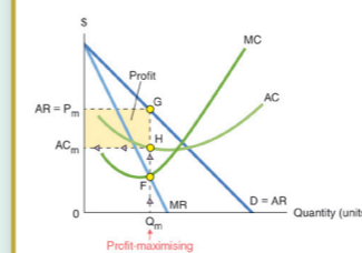
Fig. 33.16 Monopoly profit
